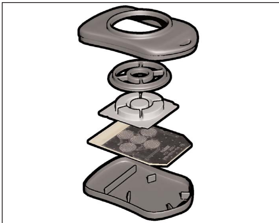
Figure 5: CMD-KEY#-*** Assembly
