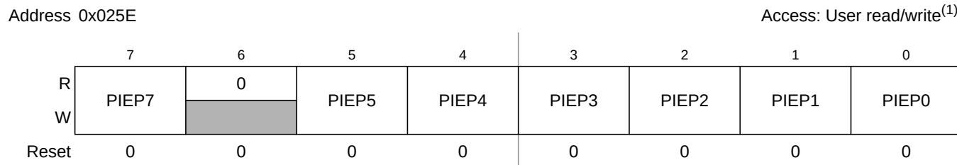
Figure 2-44. Port P Interrupt Enable Register (PIEP)
