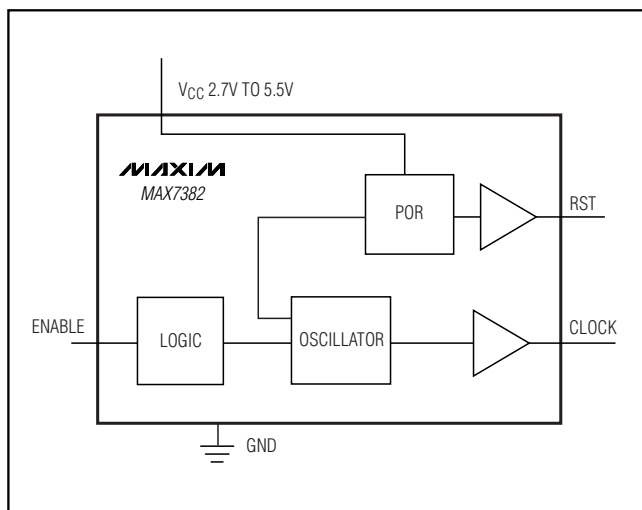
Figure 1. Functional Diagram
