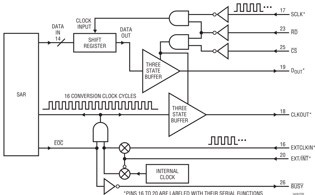
Figure 20. Functional Block Diagram for Serial Mode (SER/ \overline{\text{PAR}} = High)
