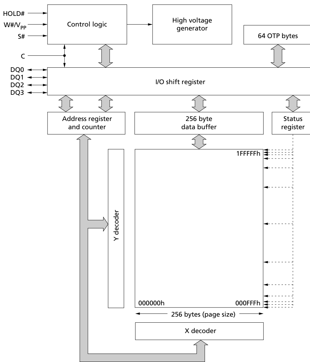
Figure 4: Block Diagram
