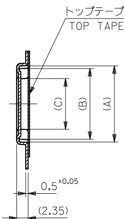
SECT. Y-Y
