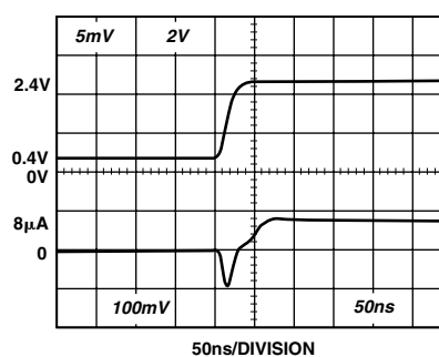
Figure 5. LSB Switching
