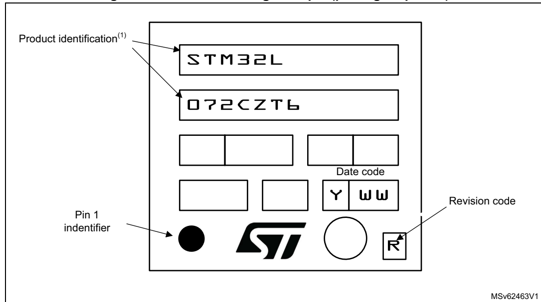
Figure 61. LQFP48 marking example (package top view)
