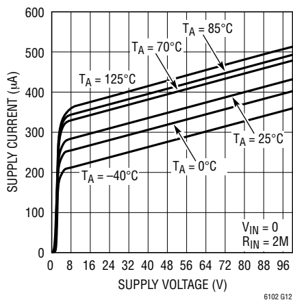
LTC6102HV: Supply Current vs Supply Voltage
