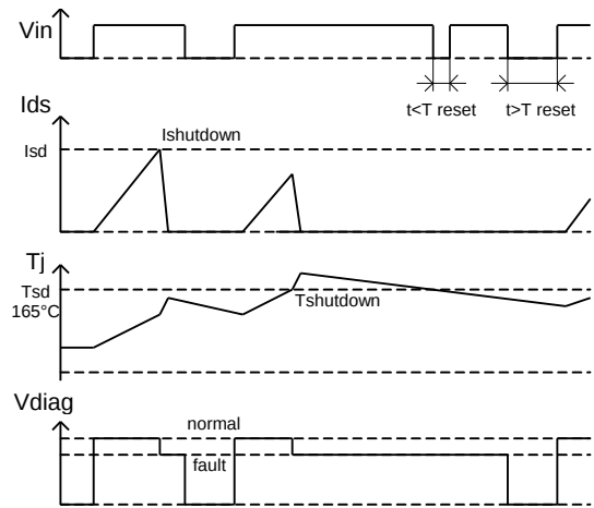
Figure 1 – Timing diagram
