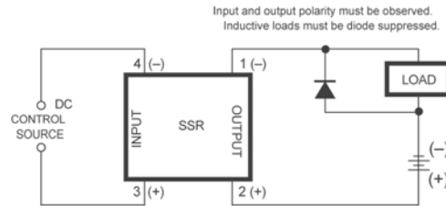
Transient Protection
