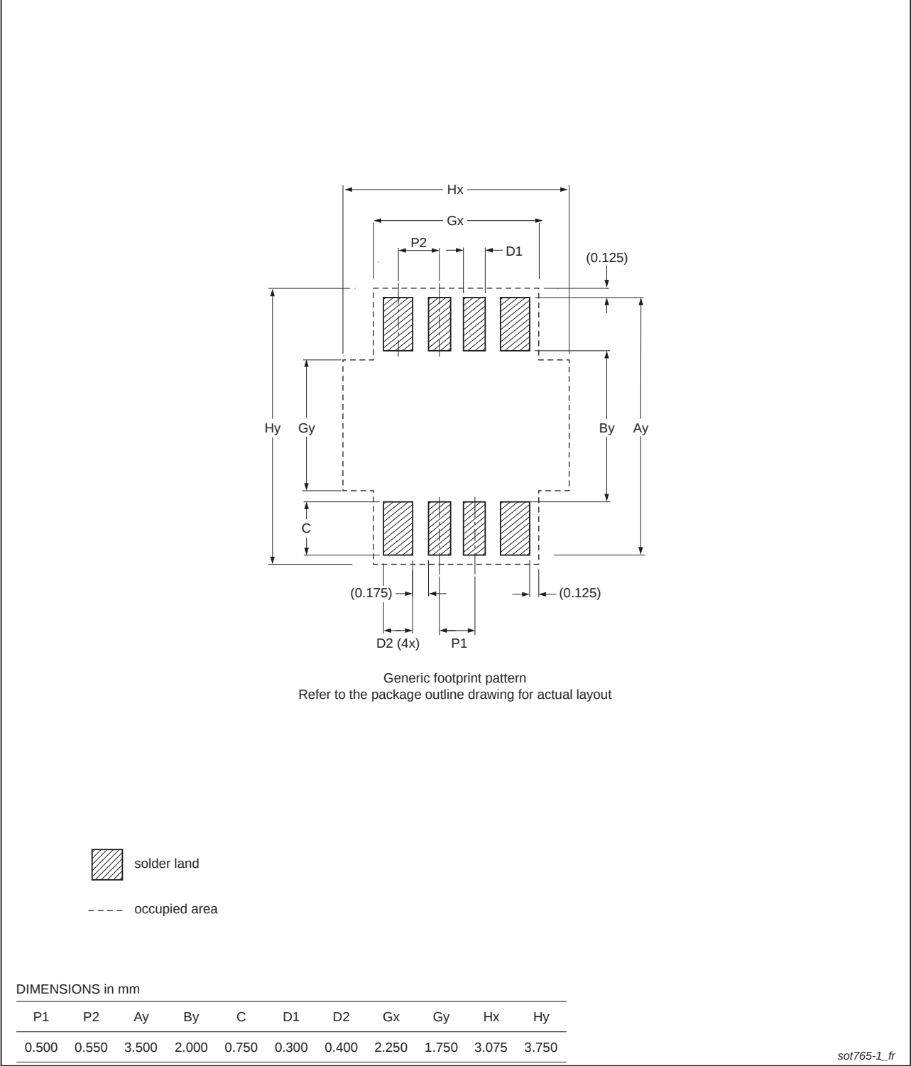
Fig 25. PCB footprint for SOT765-1 (VSSOP8); reflow soldering
