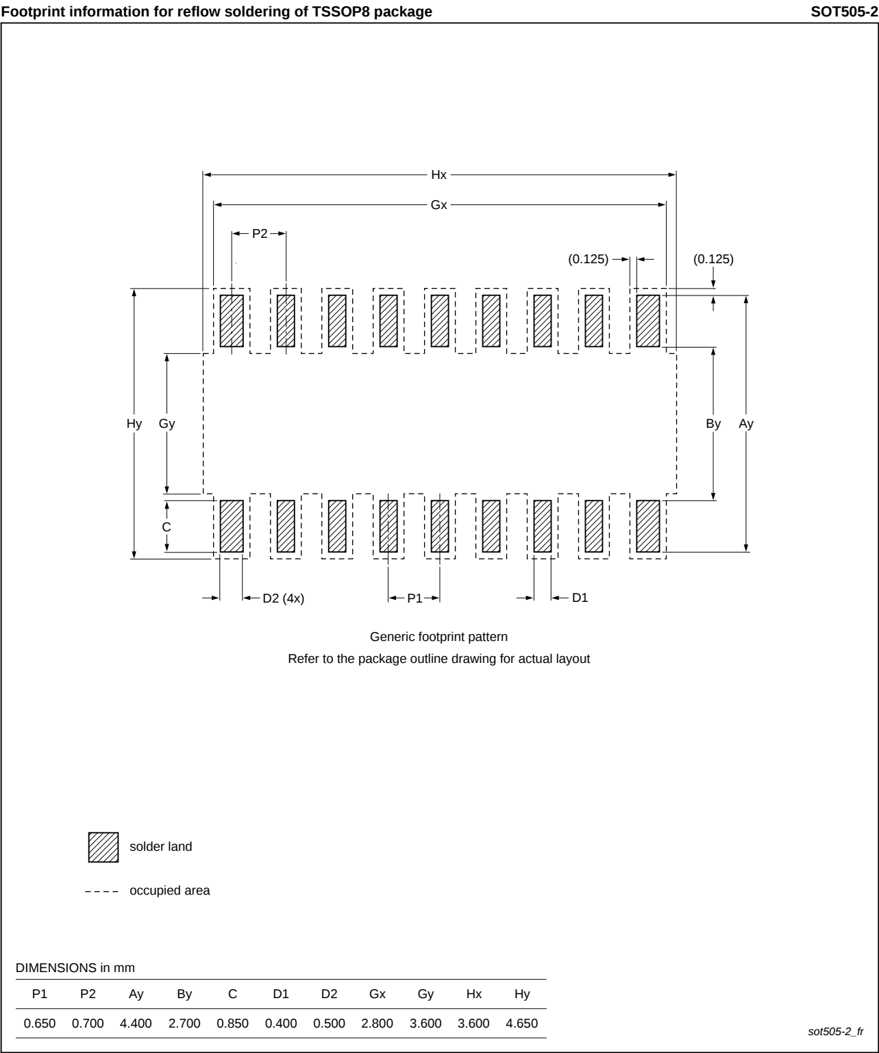
Fig 24. PCB footprint for SOT505-2 (TSSOP8); reflow soldering
