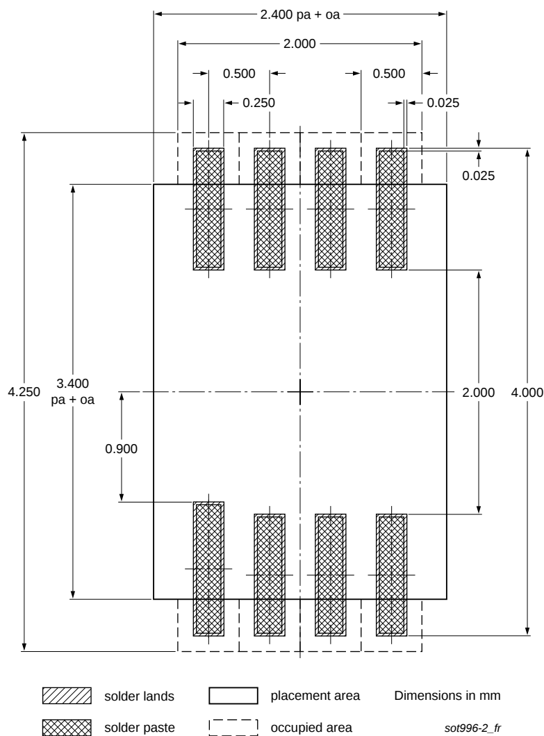
Fig 27. PCB footprint for SOT996-2 (XSON8U); reflow soldering
