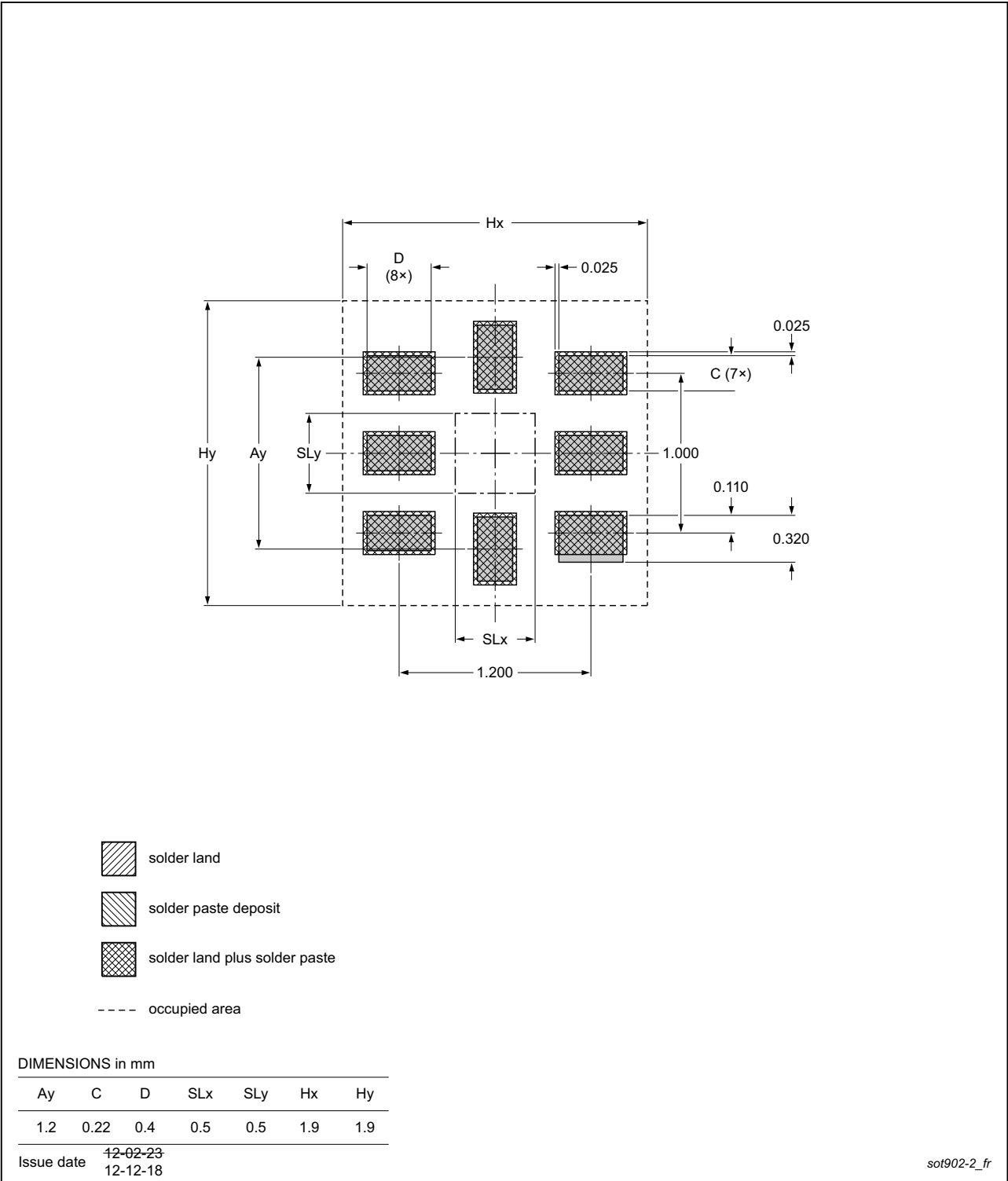
Fig 28. PCB footprint for SOT902-2 (XQFN8); reflow soldering
