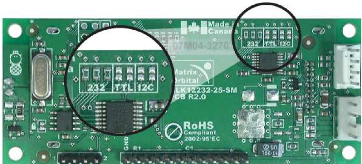
Figure 12: Protocol-Select-Jumpers
