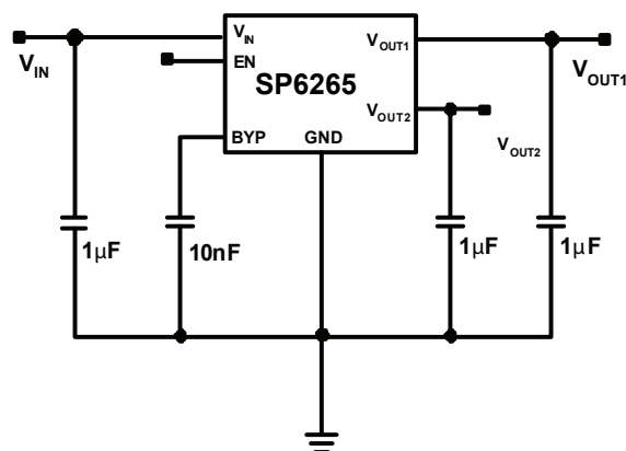
SP6265 with Bypass
