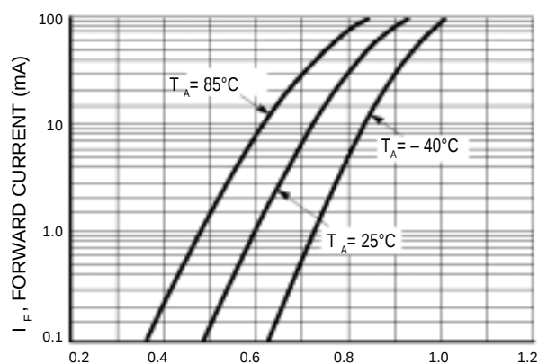
Figure 2. Forward Voltage
