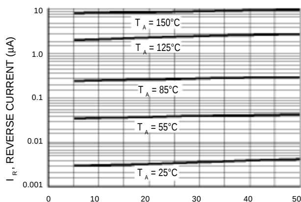
Figure 3. Leakage Current
