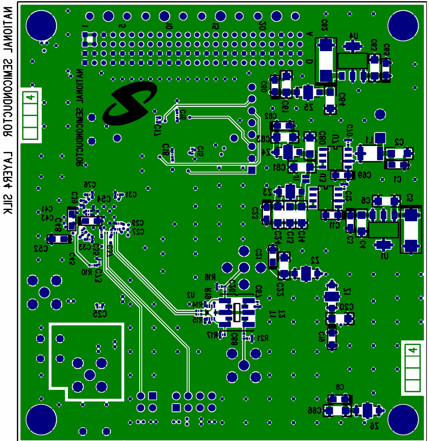
Figure 9. Layer 4 - Signal
