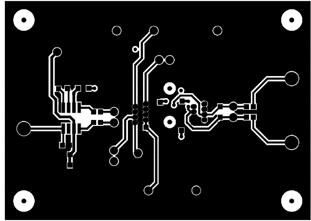
Figure 76. Wiring-Side Pattern
