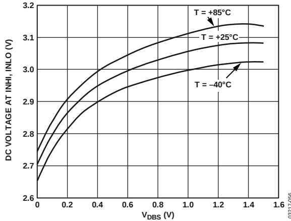
Figure 55. Common-Mode Voltage at Input Pins vs. V_{DBS} for V_S = 5\text{ V} , T = -40^{\circ}\text{C} , +25^{\circ}\text{C} , and +85^{\circ}\text{C}
