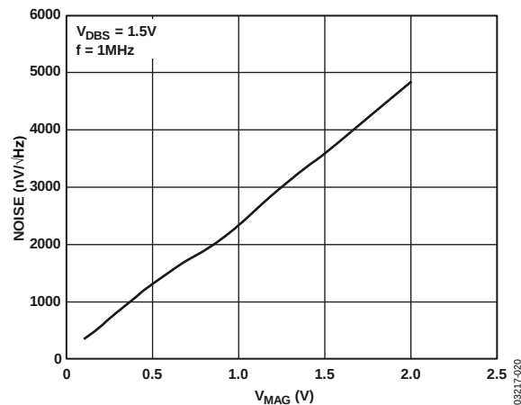
Figure 19. Output Referred Noise vs. V_{MAG}
