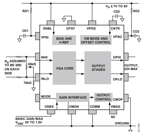
Figure 58. Input Offset Nulling in a DC-Coupled System
