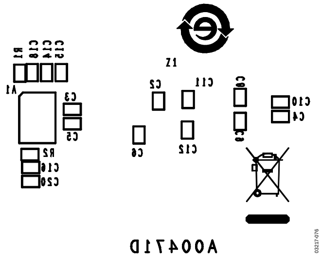
Figure 75. Wiring-Side Silkscreen
