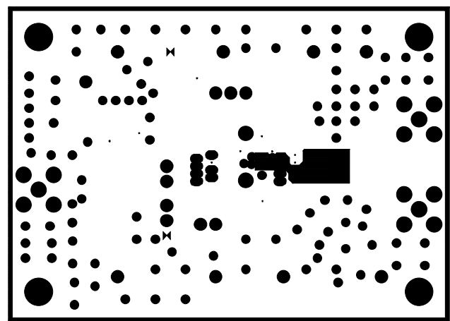
Figure 77. Inner Layer 2
