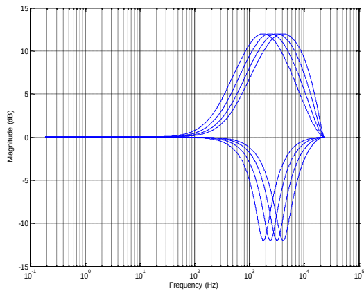
Figure 50 EQ Band 4 – Peak Filter Centre Frequencies, EQ3BW=0
