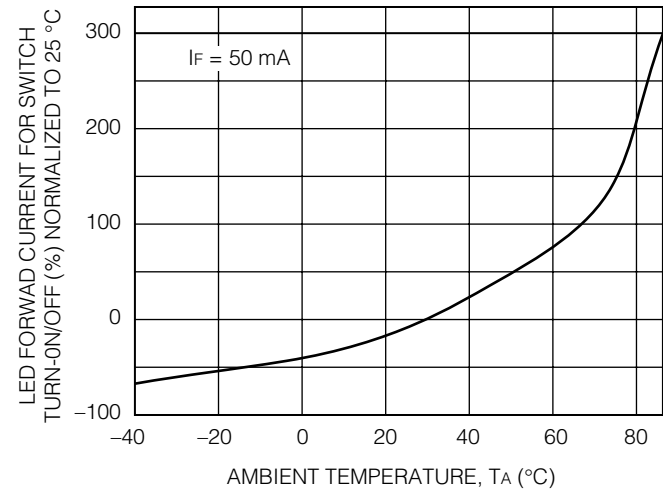
Figure 2. LED Current for Switch Turn-on/off vs. Temperature
