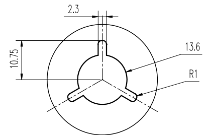
P DETAIL 6:1
