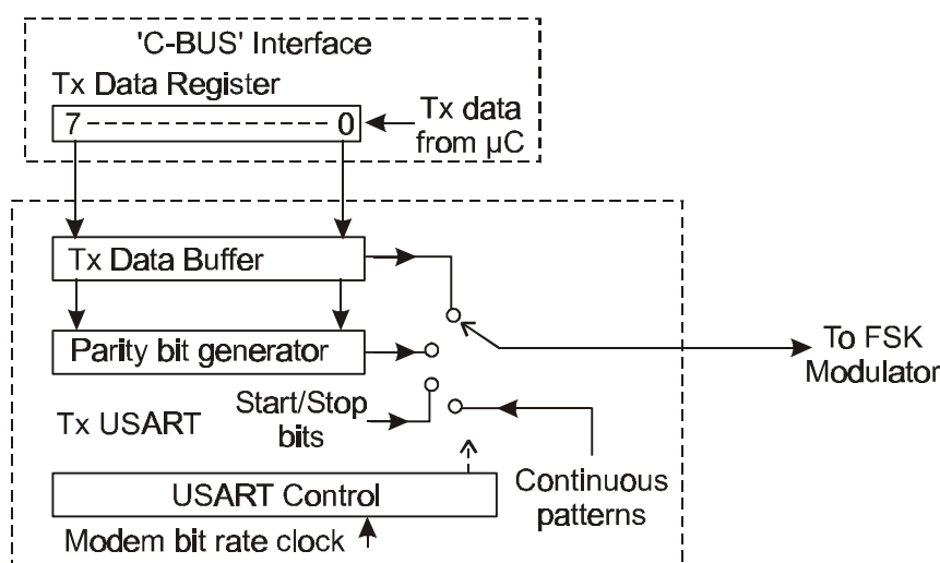
Figure 5a Tx USART
