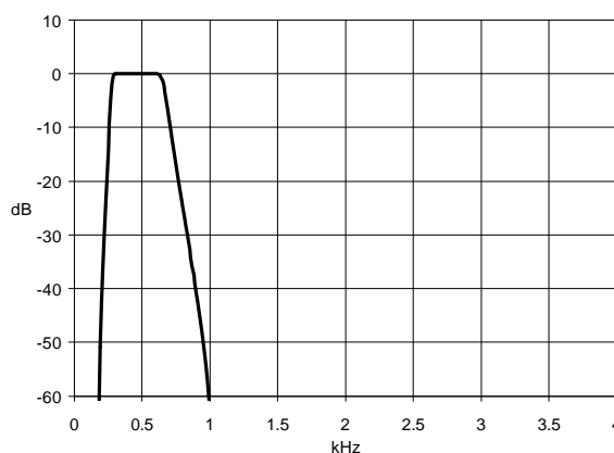
Figure 6a Response of the Call Progress Filter
