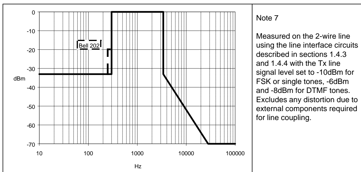
Figure 13 Maximum Out of Band Tx Line Energy Limits (see note 7)
