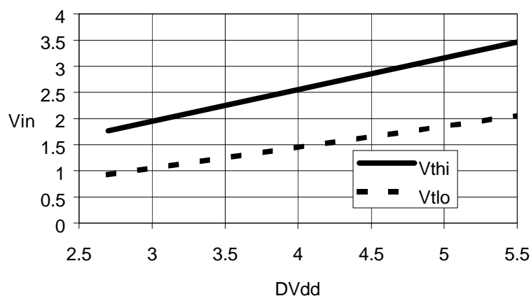
Figure 12 Typical Schmitt Trigger Input Voltage Thresholds vs. DV_{DD}
