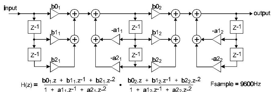
Figure 10a Programmable Tone Detectors
