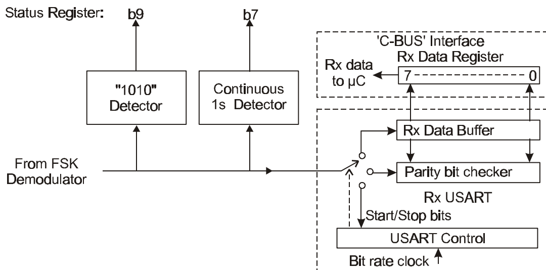
Figure 7a Rx Modem Data Paths
