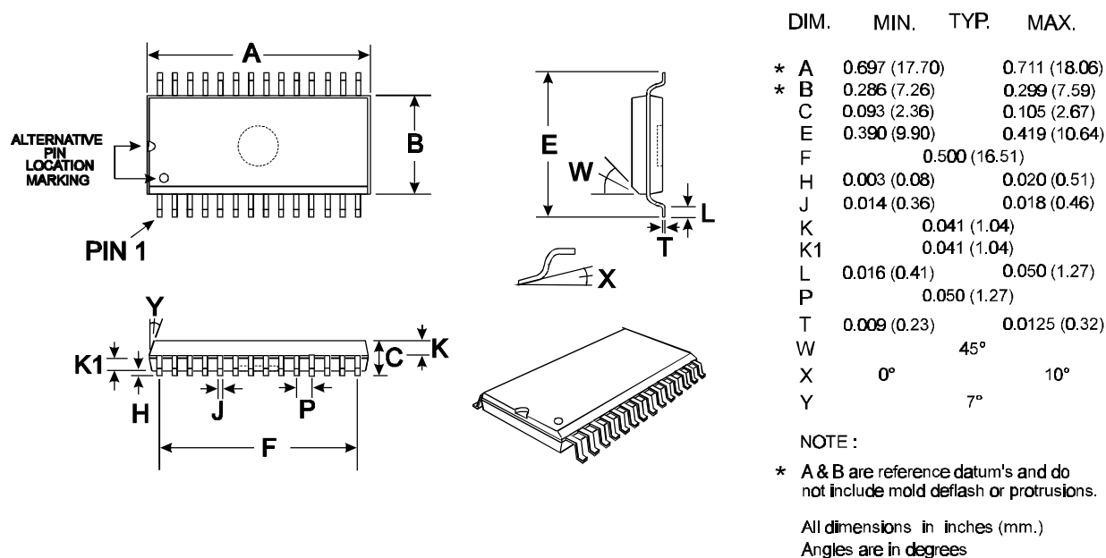
Figure 16 28-pin SOIC (D1) Mechanical Outline: Order as part no. CMX860D1
