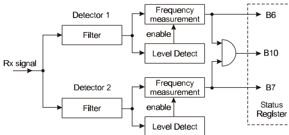
Figure 10a Programmable Tone Detectors
