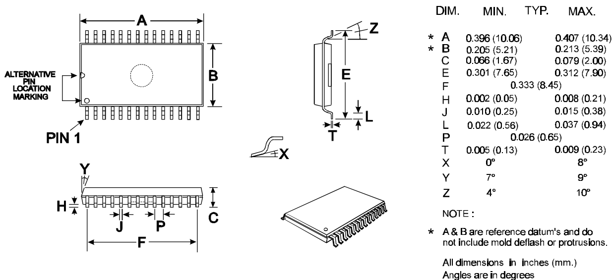
Figure 15 28-pin SSOP (D6) Mechanical Outline: Order as part no. CMX860D6
