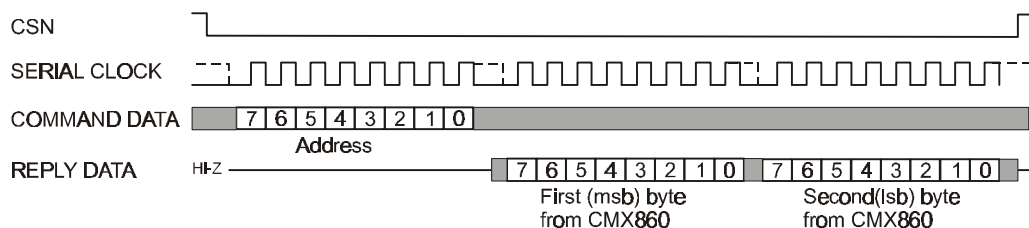
Figure 8 'C-BUS' Transactions
