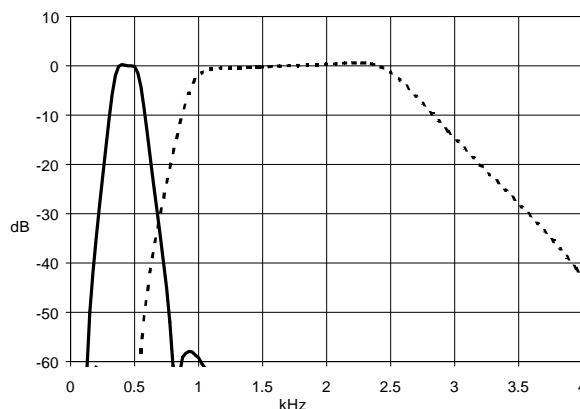
Figure 6b V.23 / Bell 202 Rx Filters
