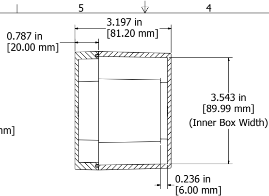
SECTION A-A End View of Assembly
