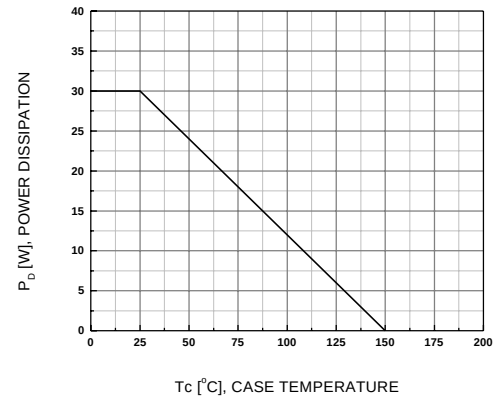
Figure 4. Power Derating
