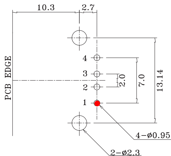
PC Board Layout - Bottom View
