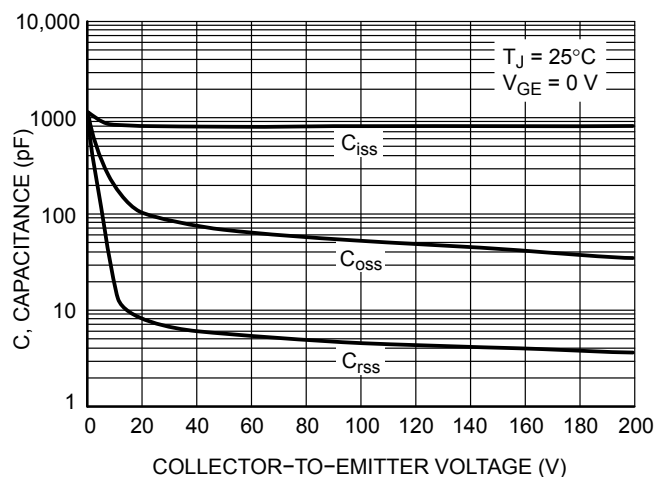
Figure 11. Capacitance Variation
