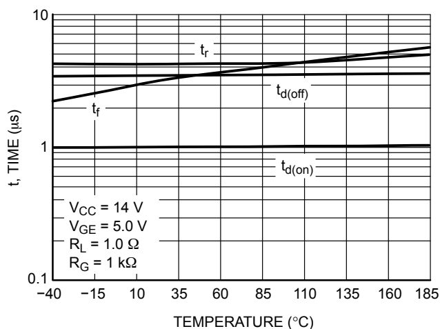
Figure 12. Resistive Switching Time Variation vs. Temperature
