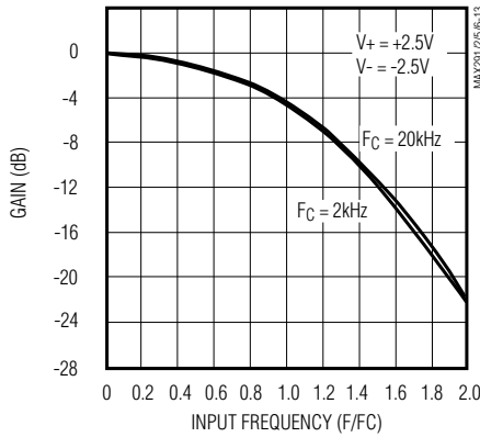
MAX296 LOW-VOLTAGE FREQUENCY RESPONSE
