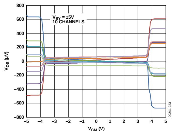
Figure 23. Input Offset Voltage ( V_{OS} ) vs. Common-Mode Voltage ( V_{CM} )
