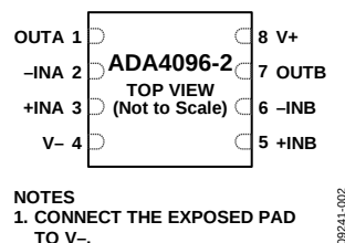
Figure 2. 8-Lead LFCSP (CP-8-10), ADA4096-2
