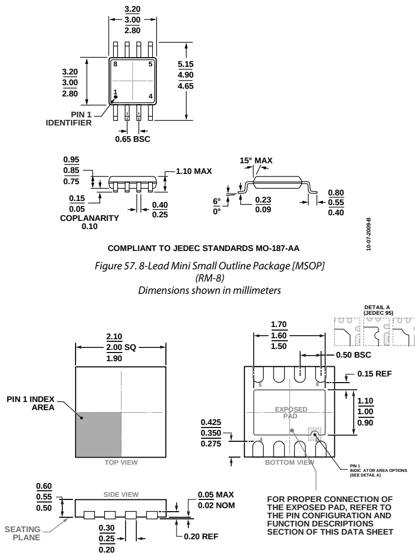
Figure 58. 8-Lead Lead Frame Chip Scale Package [LFCSP] 2 mm x 2 mm Body and 0.55 mm Package Height (CP-8-10)
