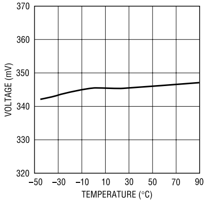
Battery Present Threshold Voltage (per Cell)
