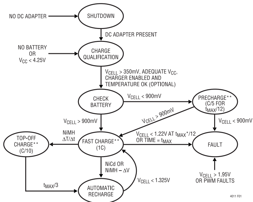
Figure 1. LTC4011 State Diagram
