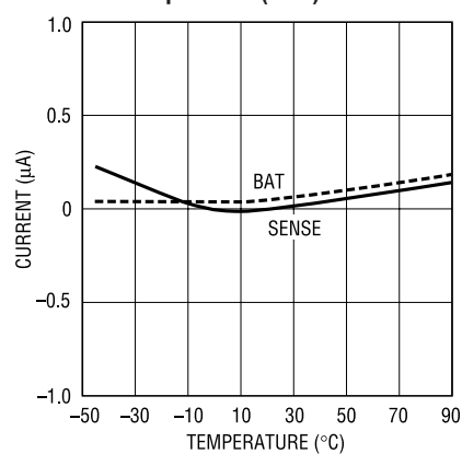
PWM Input Bias (OFF)
