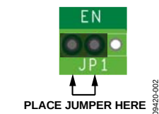
Figure 2. SD Jumper Position
