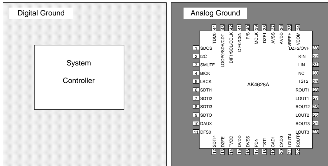
Figure 26. Ground Layout
