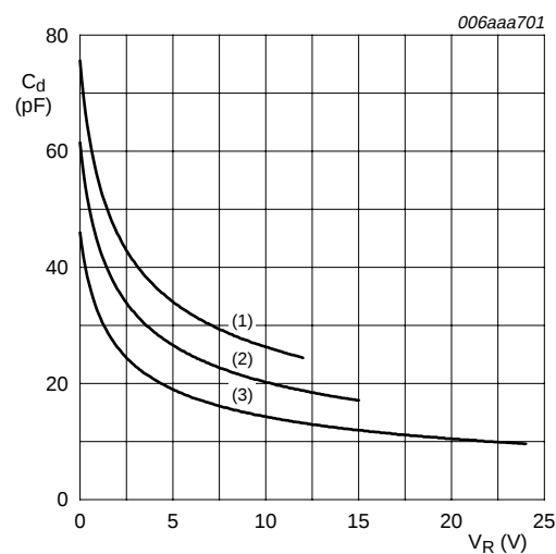
f = 1 \text{ MHz}; T_{\text{amb}} = 25^\circ\text{C} (1) PESD12VS5UD (2) PESD15VS5UD (3) PESD24VS5UD
