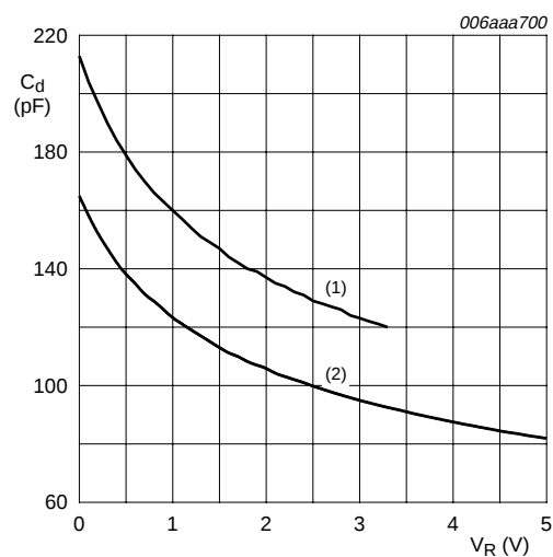
f = 1 \text{ MHz}; T_{\text{amb}} = 25^\circ\text{C} (1) PESD3V3S5UD (2) PESD5V0S5UD
