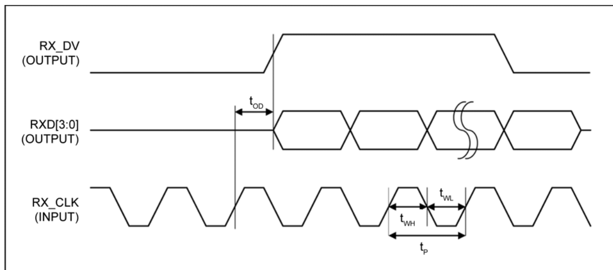
Figure 23. MII Receive Timing in MAC Mode
