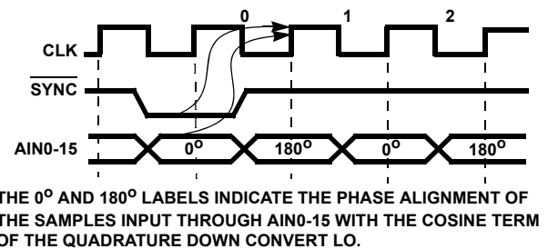
FIGURE 17. DATA SYNCHRONIZATION WITH PHASE OF DOWN CONVERT LO
