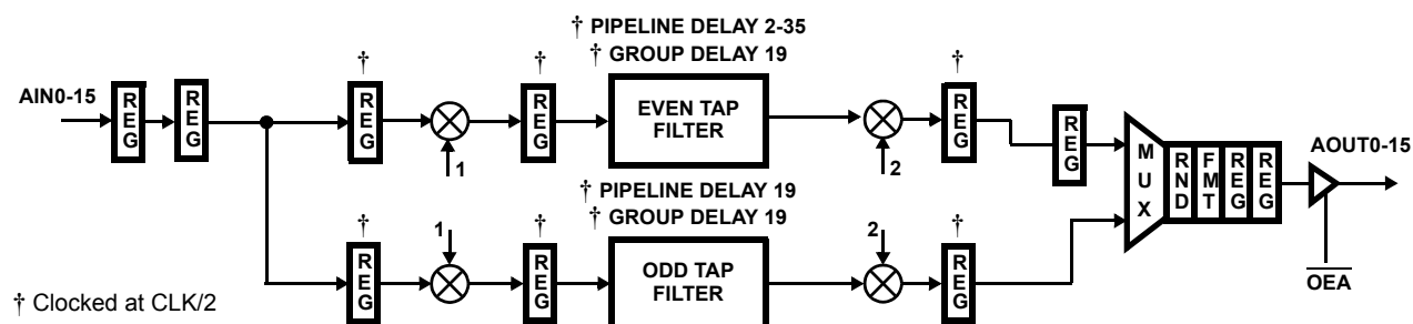
FIGURE 11A. DATA FLOW DIAGRAM FOR INTERPOLATE BY 2 FILTER MODE (INT/EXT = 1)
