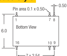
16 Pin SMD Package
