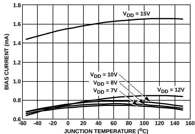
FIGURE 6. OFF-STATE I XHB BIAS CURRENT
