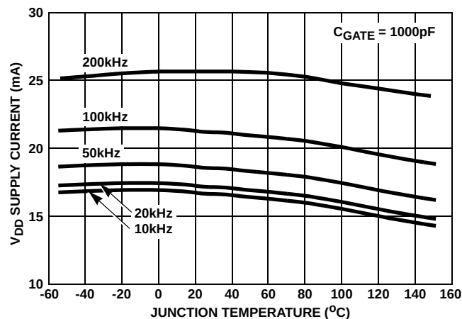
FIGURE 4. V DD SUPPLY CURRENT vs SWITCHING FREQUENCY
