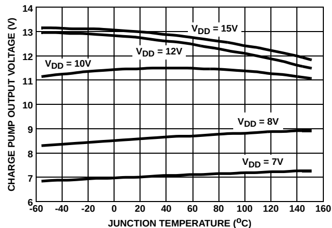
FIGURE 8. CHARGE PUMP OUTPUT VOLTAGE
