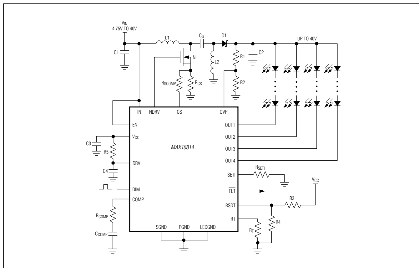
Figure 5. SEPIC Configuration
