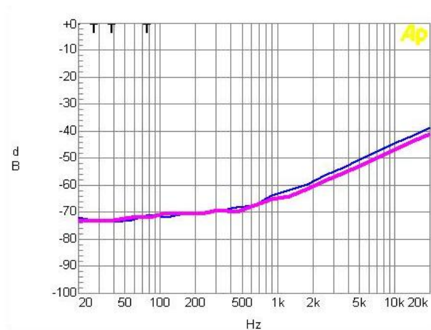
Figure 15 PSRR vs. Frequency VDD=5V, RL=8ohm, BTL, Input AC-grounded
