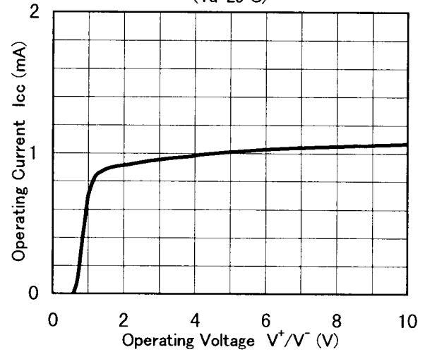
Operating Current vs. Operating Voltage ( T_a = 25^\circ C )
