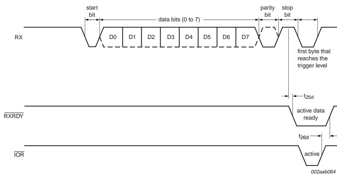
Fig 20. Receive ready timing in FIFO mode
