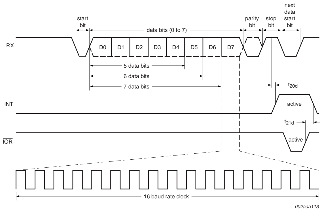
Fig 18. Receive timing
