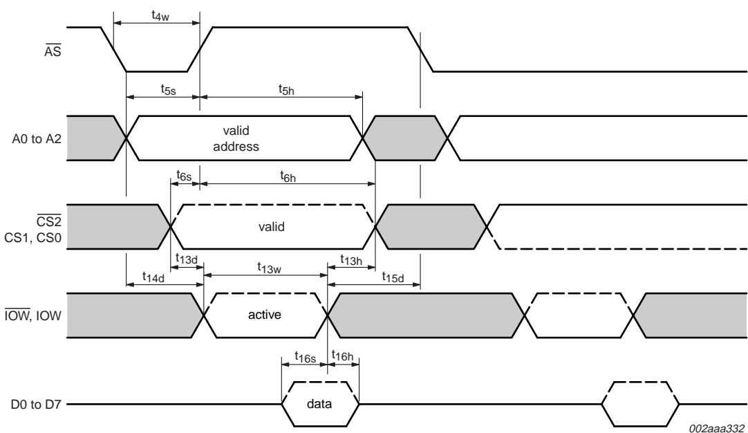
Fig 13. General write timing when using AS signal
