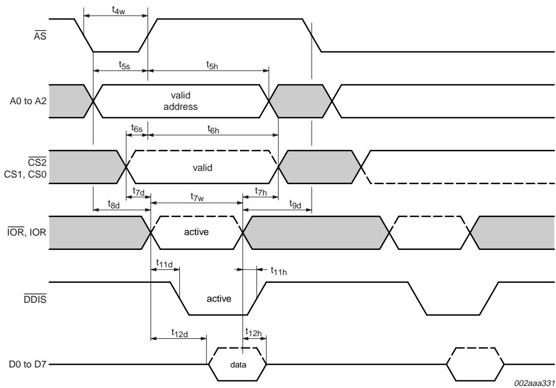
Fig 12. General read timing when using AS signal
