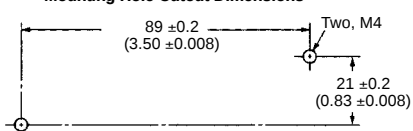
Mounting Hole Cutout Dimensions
