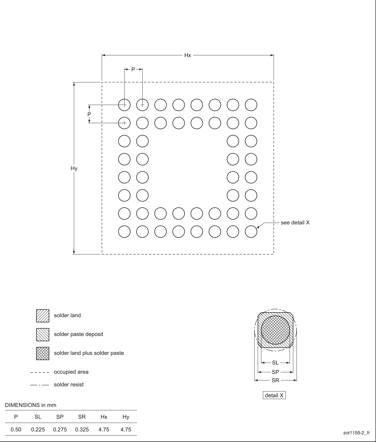
Fig 43. Reflow soldering for the TFBGA48 package
