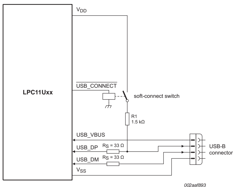
Fig 29. USB interface with soft-connect
