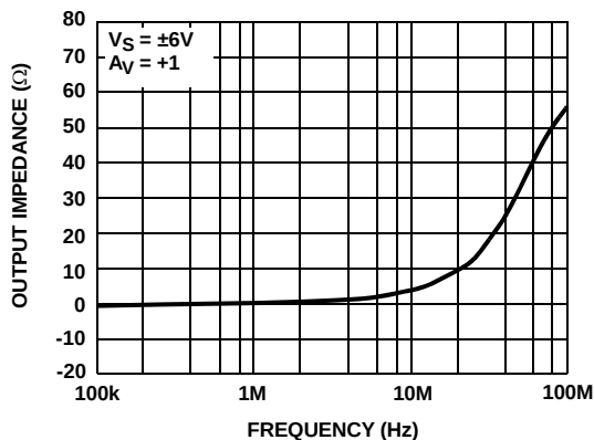
FIGURE 4. CLOSED LOOP OUTPUT IMPEDANCE vs FREQUENCY
