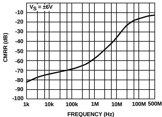
FIGURE 6. CMRR
