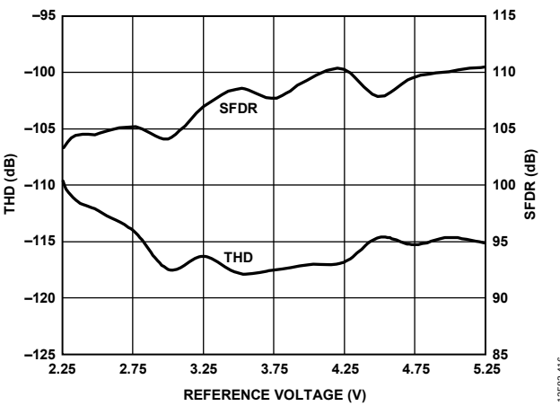
Figure 20. THD and SFDR vs. Reference Voltage
