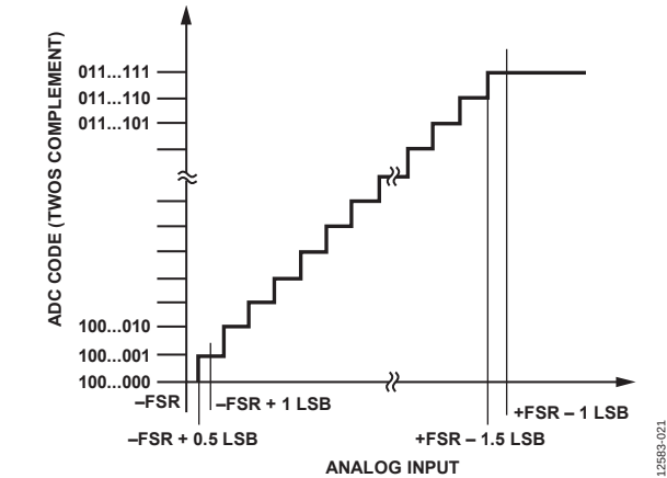
Figure 29. ADC Ideal Transfer Function
