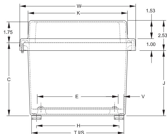
End View
