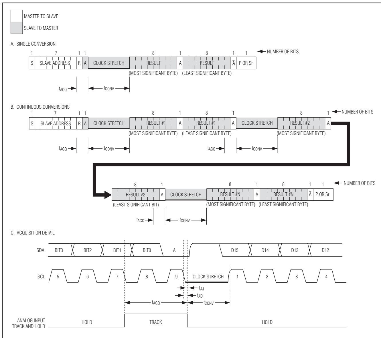
Figure 11. Read Cycle
