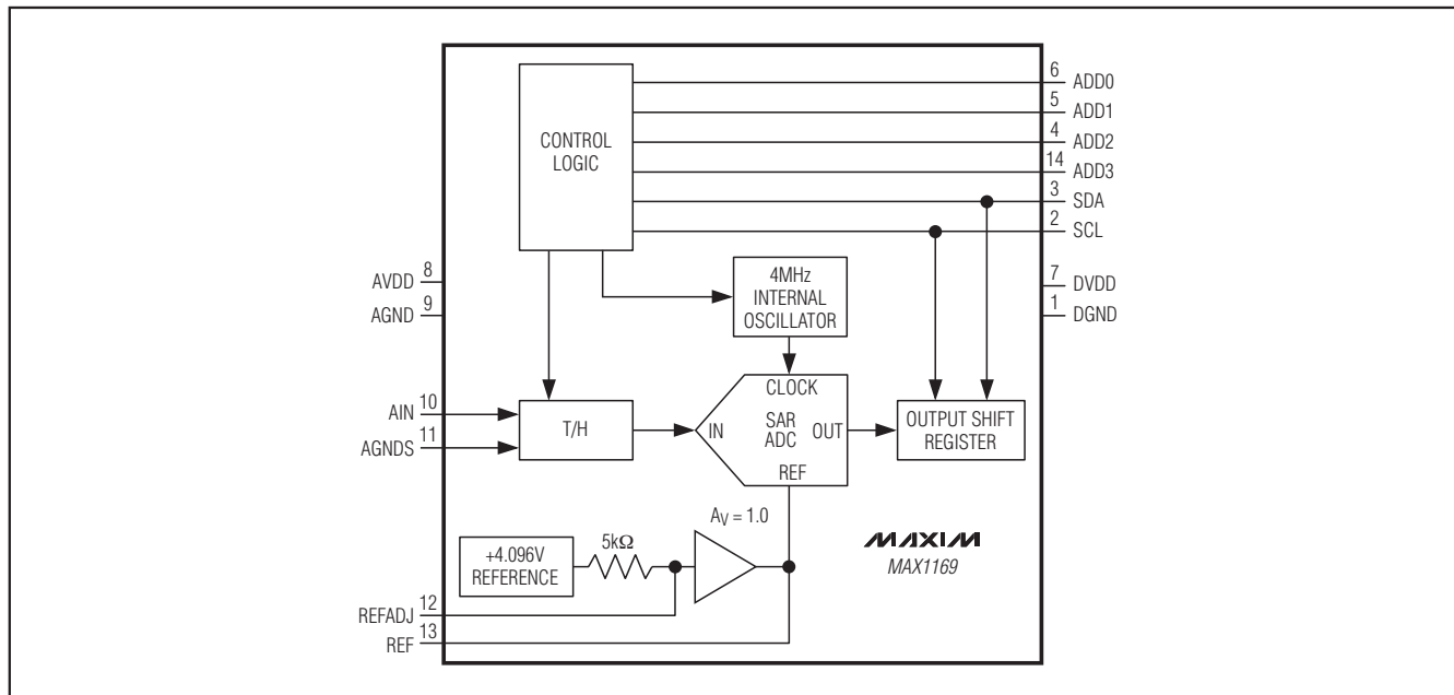
Figure 3. MAX1169 Simplified Functional Diagram
