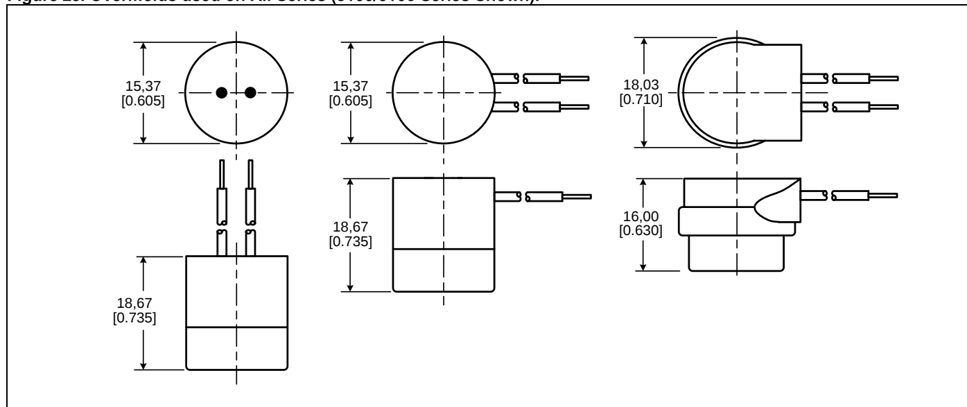
Figure 29. Overmolds used on All Series (3100/3106 Series Shown).
