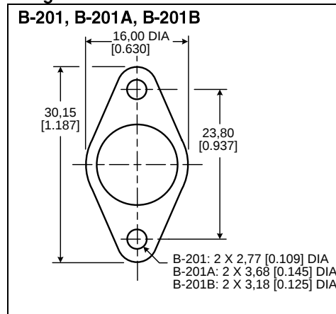
Figure 19. 3001/3004 Brackets
