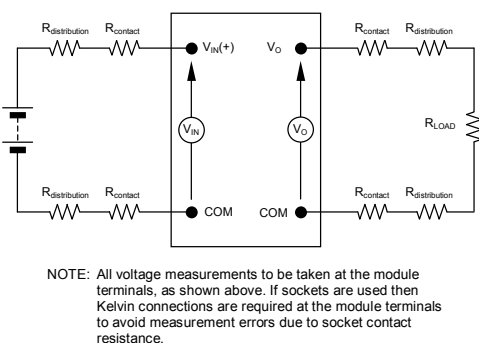
Figure 45. Output Voltage and Efficiency Test Setup.
