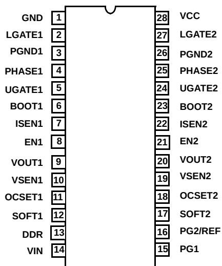
ISL6444 (28 LD QSOP) TOP VIEW
