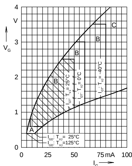
Fig. 1 Gate voltage and gate current Triggering:
