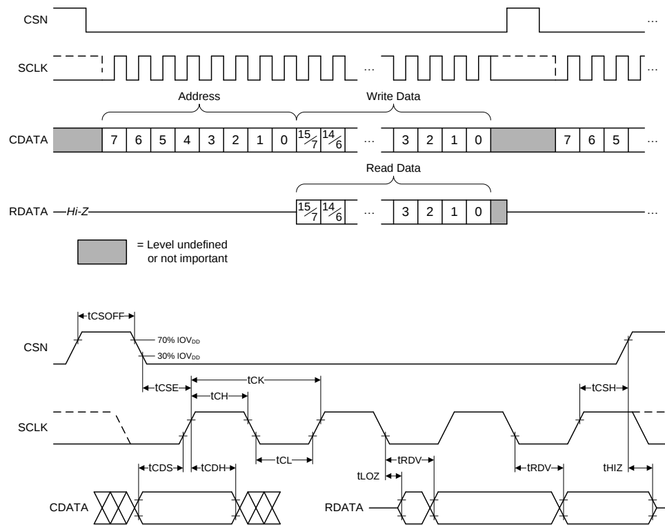
Figure 31 C-BUS Timings
