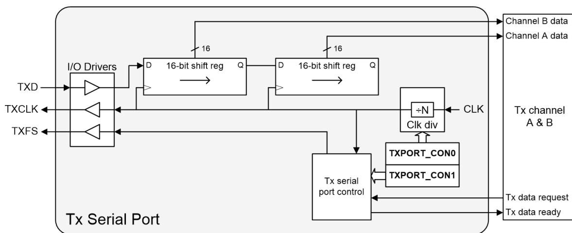
Figure 18 Tx Serial Port
